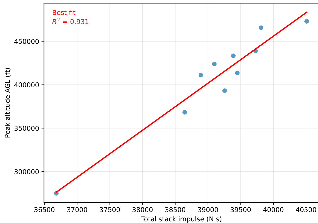
Stage impulse and mass sensitivity of apogee
